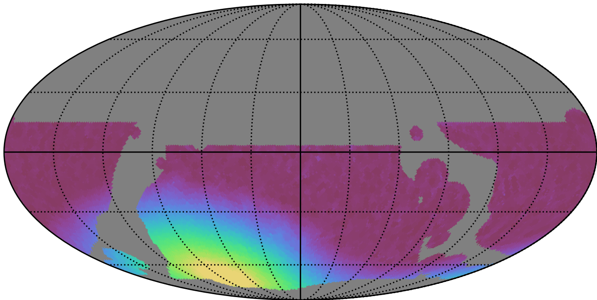
baseline_v3.5_10yrs WFD z band: Min moonDistance
