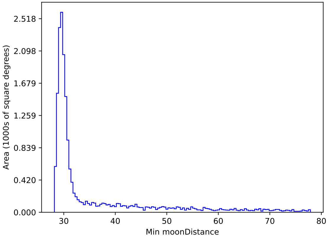
baseline_v3.5_10yrs WFD z band: Min moonDistance
