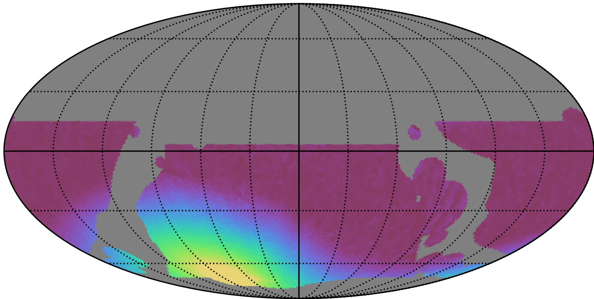
baseline_v3.5_10yrs WFD y band: Min moonDistance
