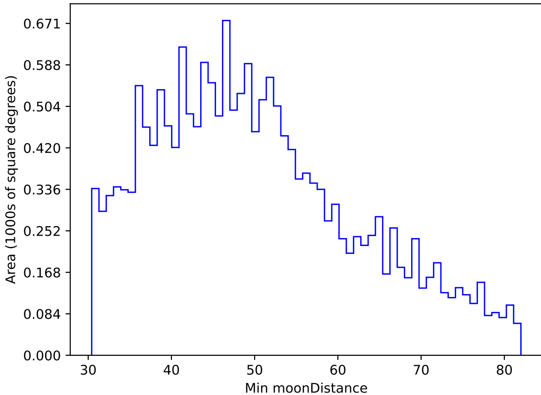
baseline_v3.5_10yrs WFD u band: Min moonDistance
