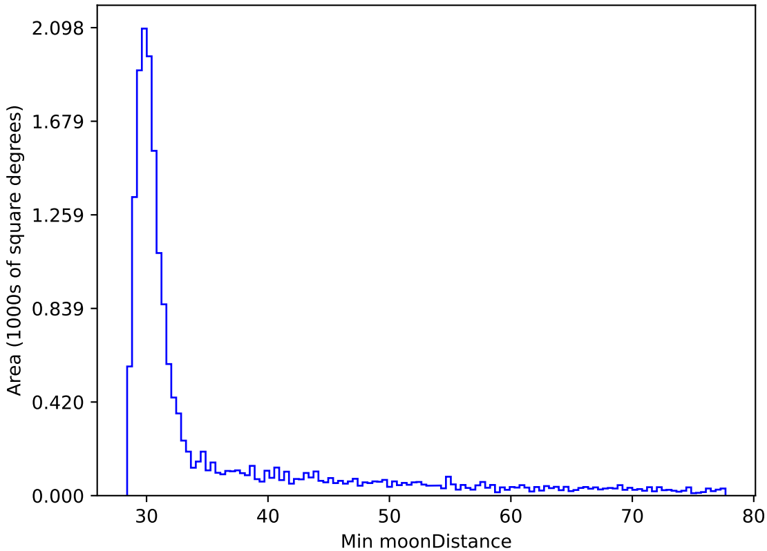
baseline_v3.5_10yrs WFD i band: Min moonDistance
