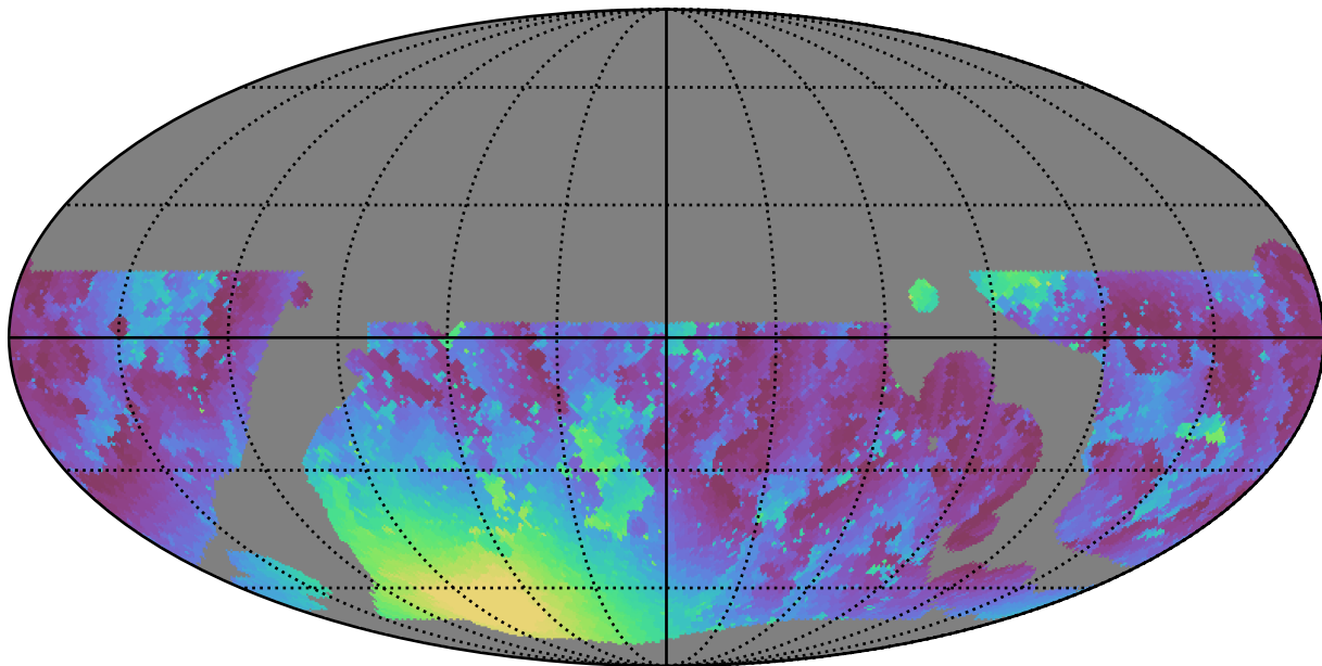
baseline_v3.5_10yrs WFD g band: Min moonDistance
