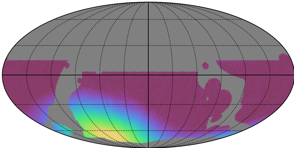
baseline_v3.5_10yrs WFD all bands: Min moonDistance
