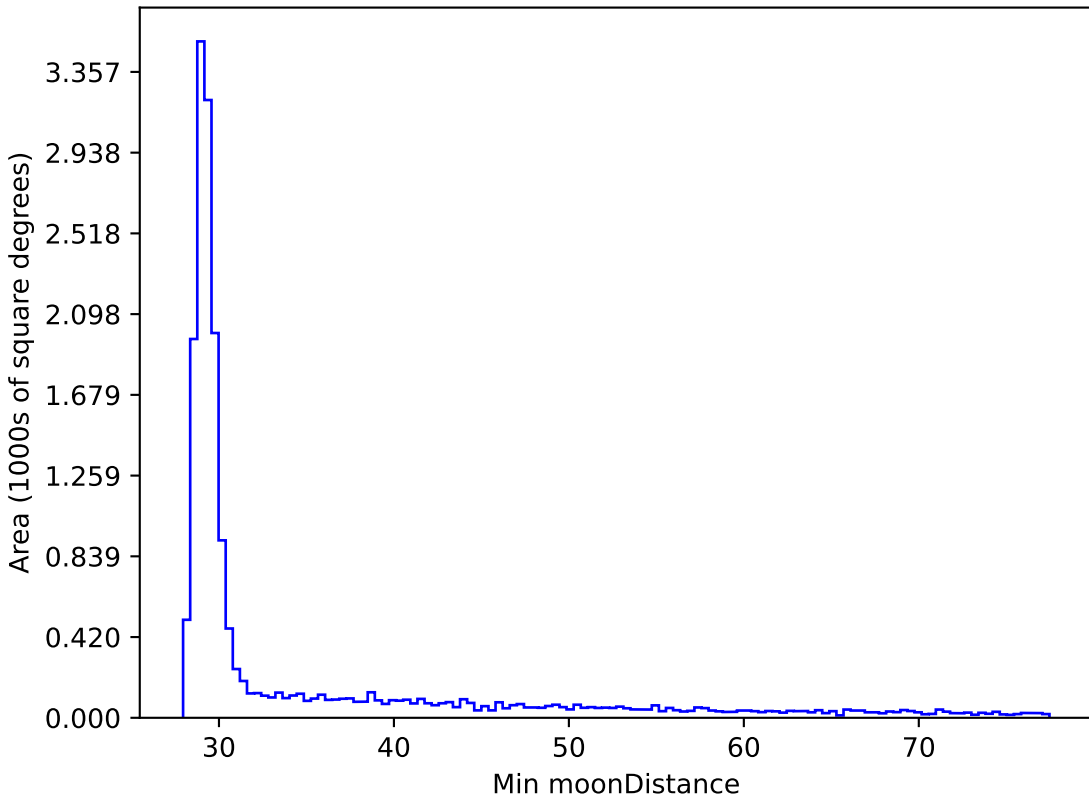
baseline_v3.5_10yrs WFD all bands: Min moonDistance
