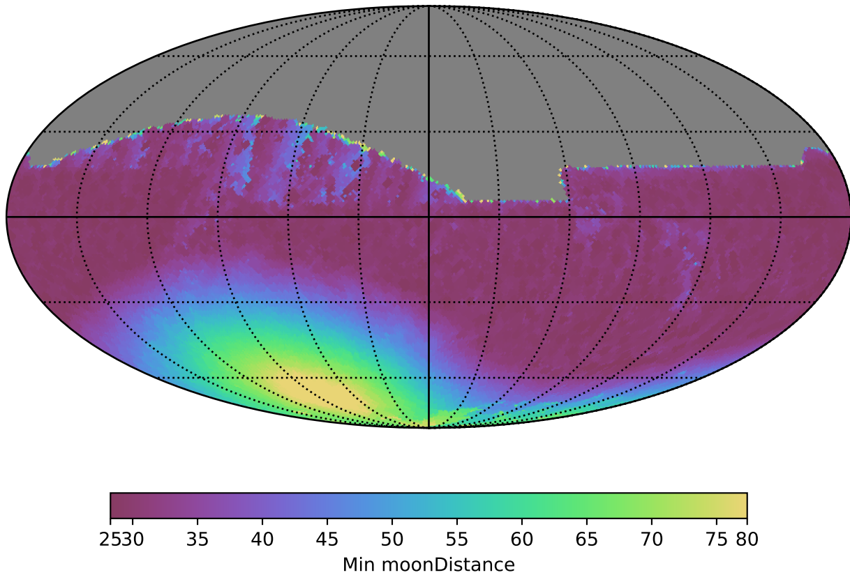
baseline_v3.5_10yrs All sky z band: Min moonDistance
