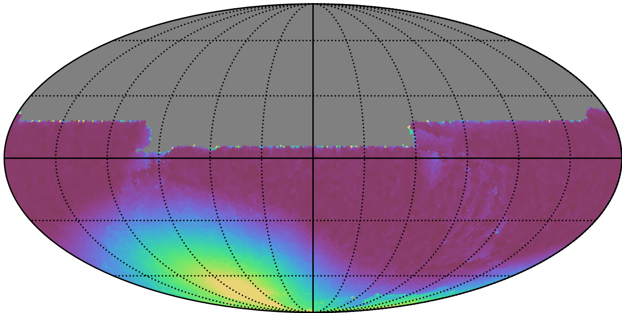
baseline_v3.5_10yrs All sky y band: Min moonDistance
