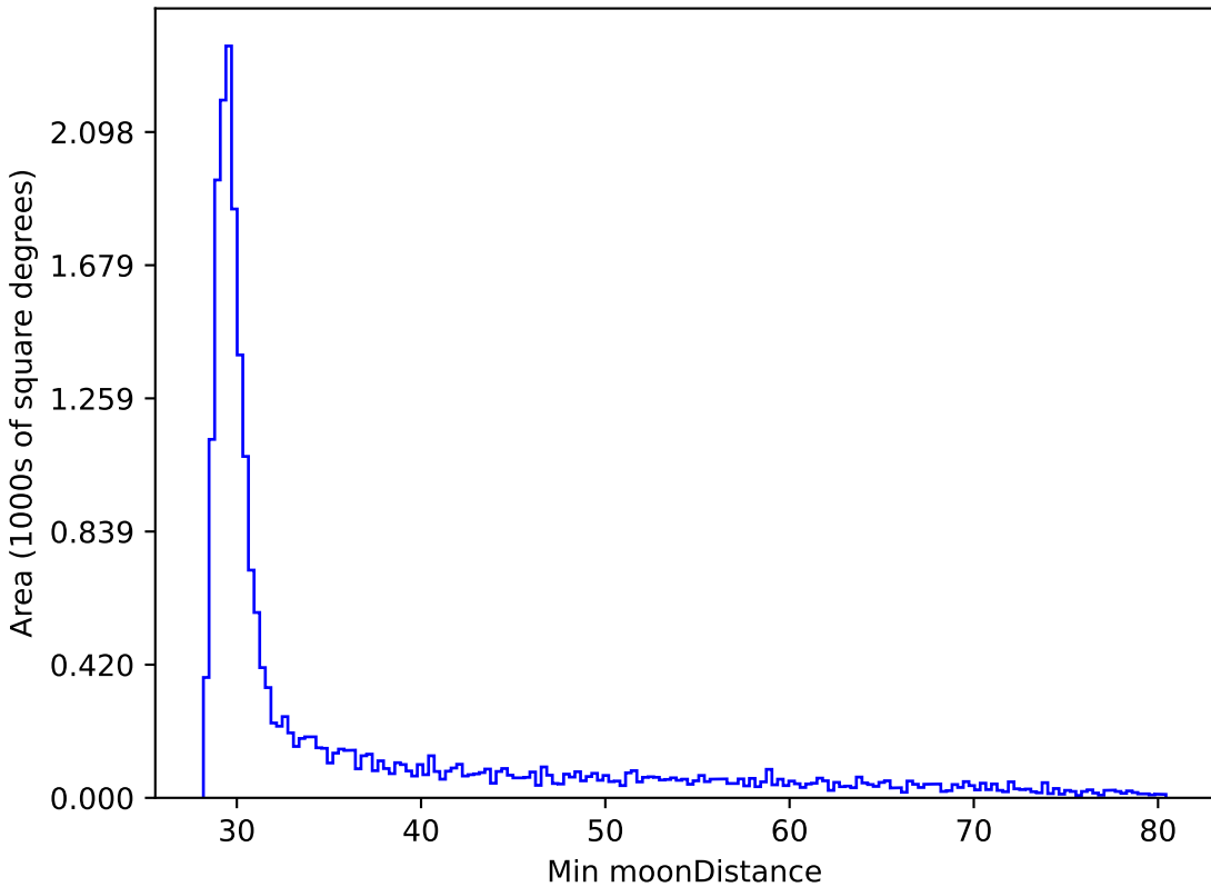
baseline_v3.5_10yrs All sky y band: Min moonDistance
