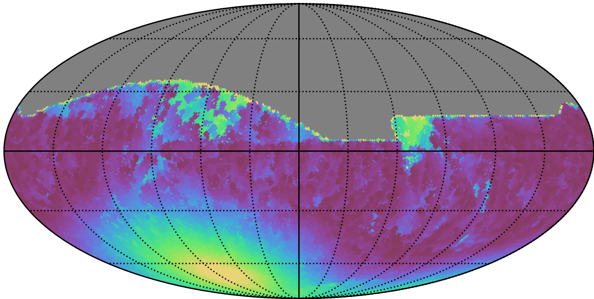
baseline_v3.5_10yrs All sky r band: Min moonDistance
