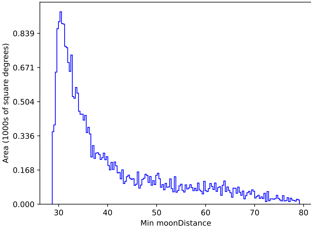
baseline_v3.5_10yrs All sky r band: Min moonDistance
