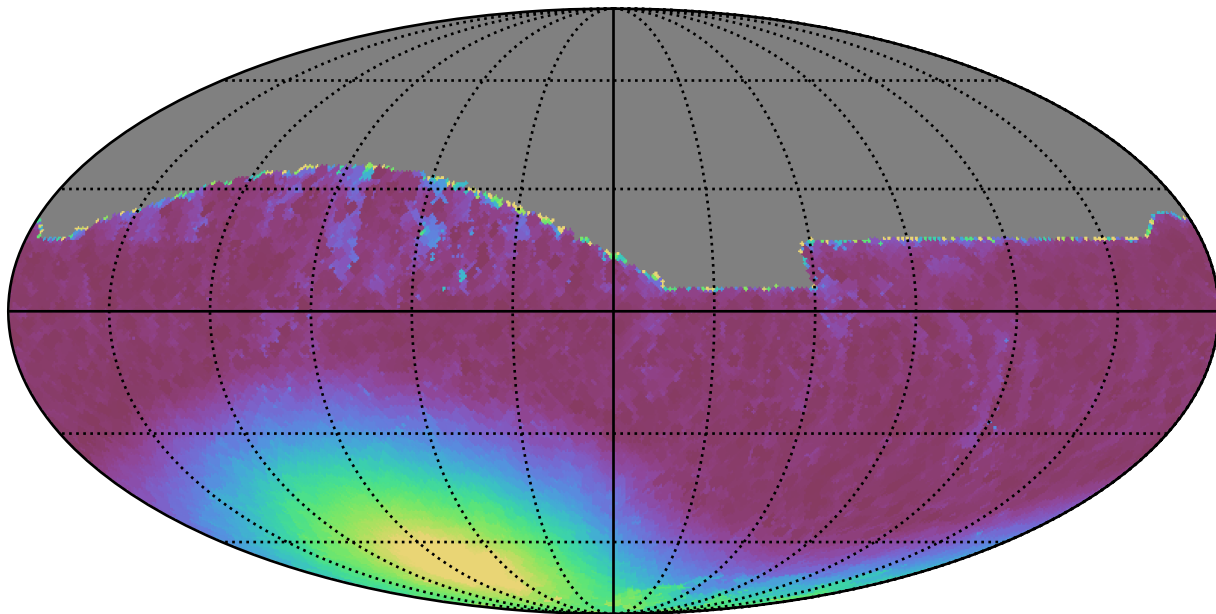
baseline_v3.5_10yrs All sky i band: Min moonDistance
