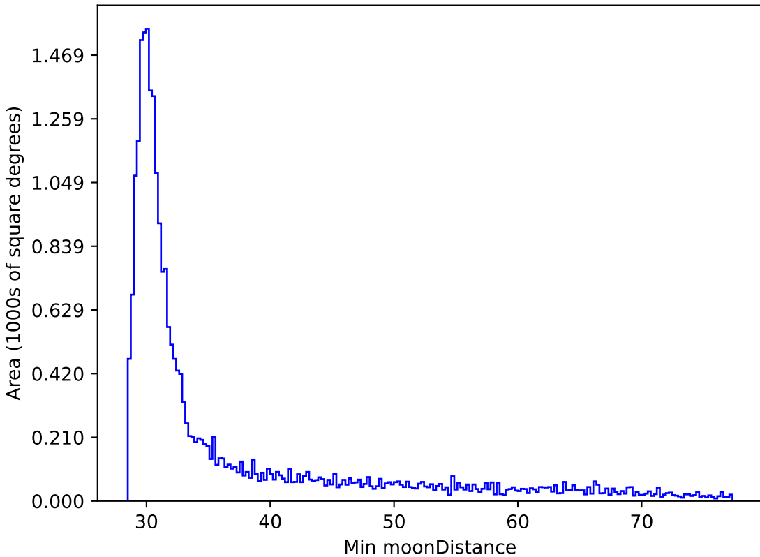
baseline_v3.5_10yrs All sky i band: Min moonDistance
