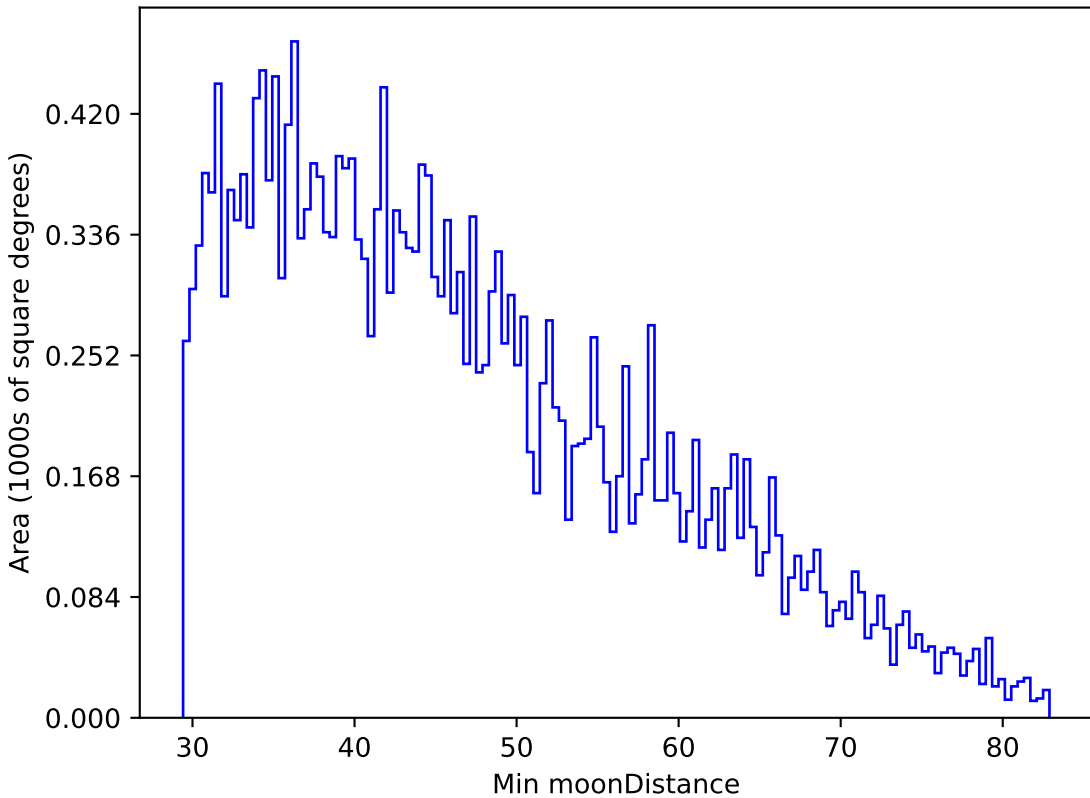
baseline_v3.5_10yrs All sky g band: Min moonDistance
