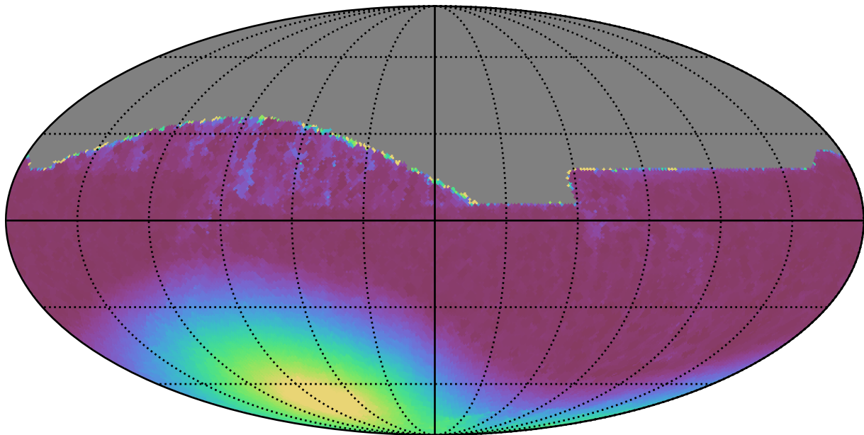
baseline_v3.5_10yrs All sky all bands: Min moonDistance
