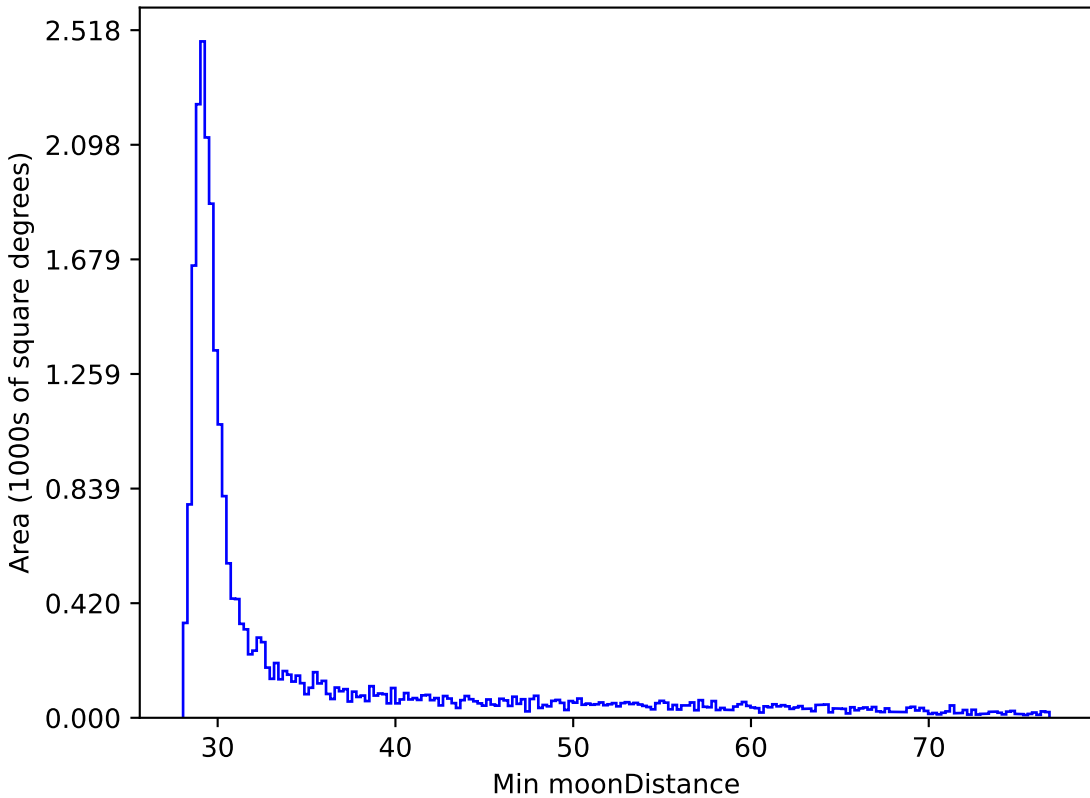
baseline_v3.5_10yrs All sky all bands: Min moonDistance
