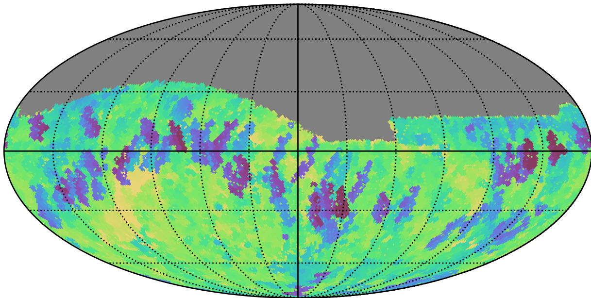
baseline_v3.5_10yrs Yr 1 z band: Min fiveSigmaDepth
