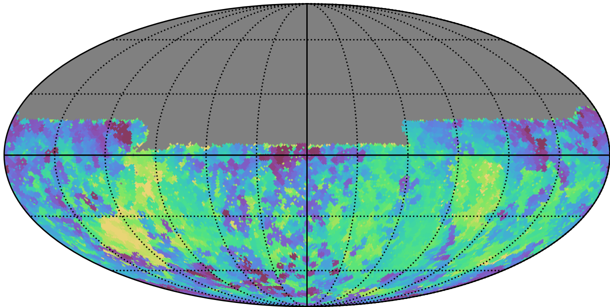
baseline_v3.5_10yrs Yr 1 y band: Min fiveSigmaDepth
