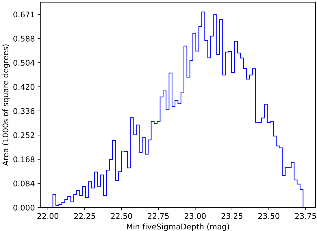
baseline_v3.5_10yrs Yr 1 u band: Min fiveSigmaDepth
