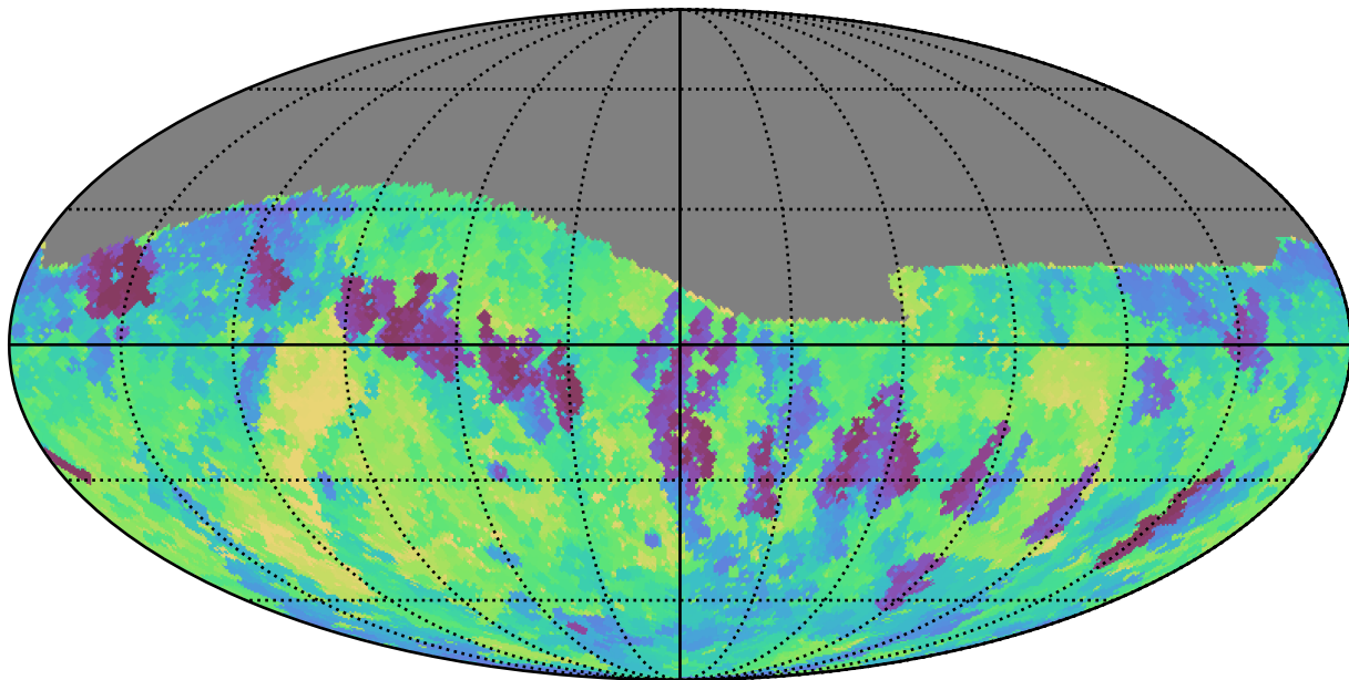
baseline_v3.5_10yrs Yr 1 r band: Min fiveSigmaDepth
