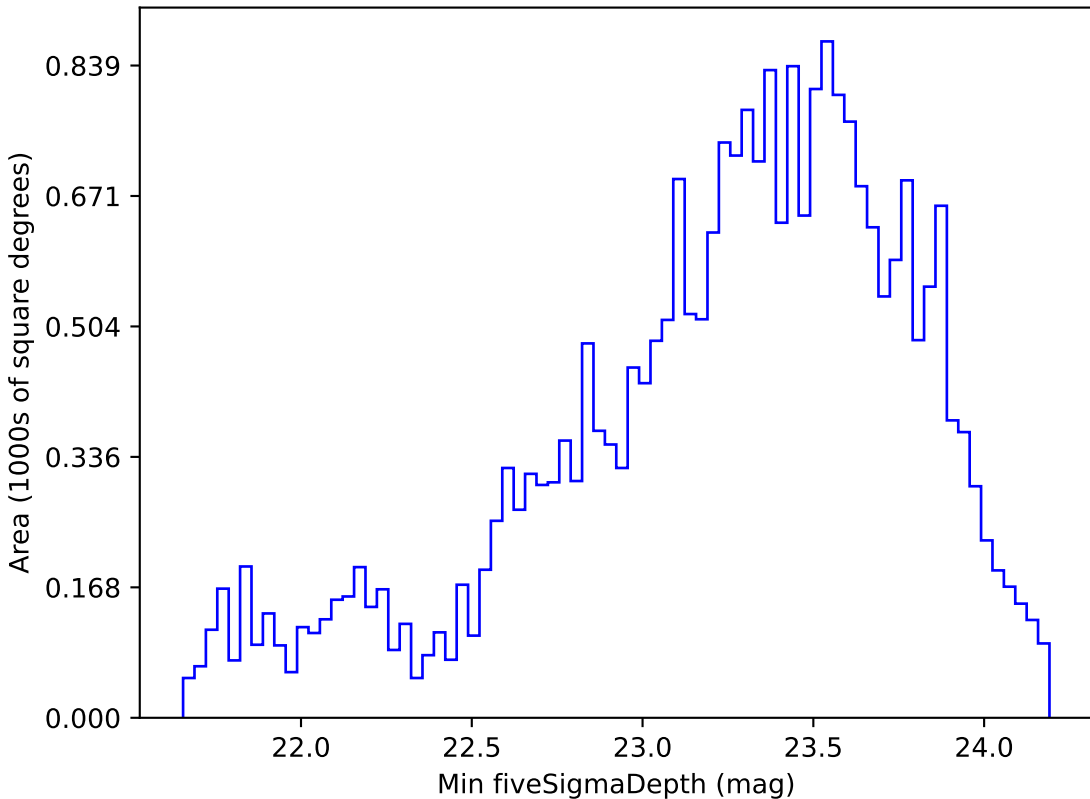
baseline_v3.5_10yrs Yr 1 r band: Min fiveSigmaDepth
