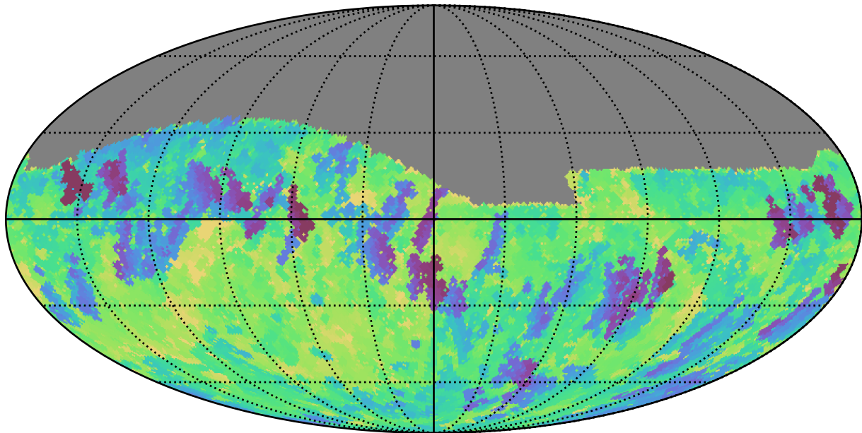
baseline_v3.5_10yrs Yr 1 i band: Min fiveSigmaDepth
