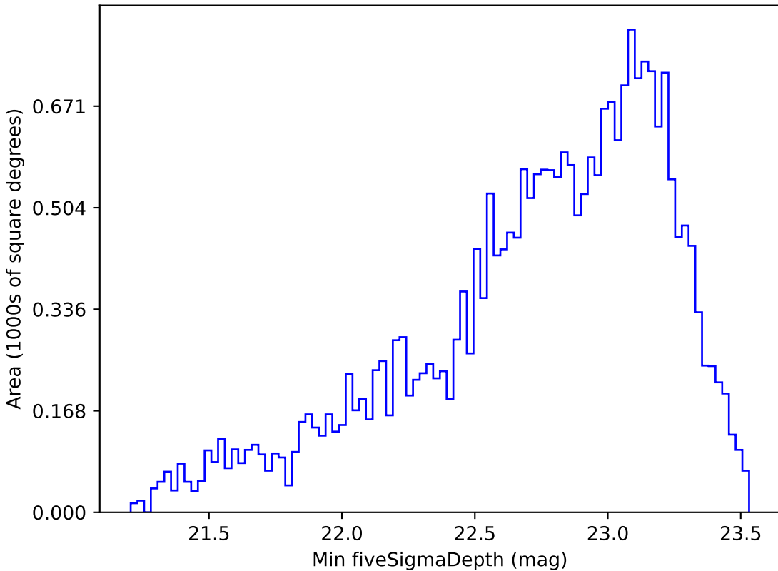
baseline_v3.5_10yrs Yr 1 i band: Min fiveSigmaDepth
