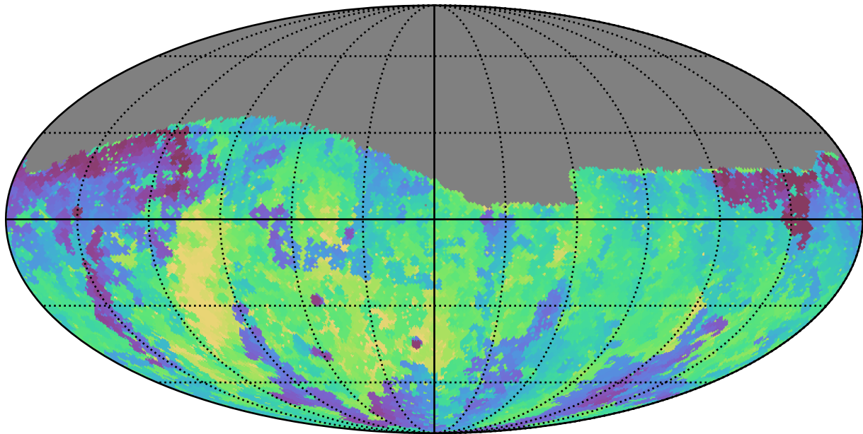
baseline_v3.5_10yrs Yr 1 g band: Min fiveSigmaDepth
