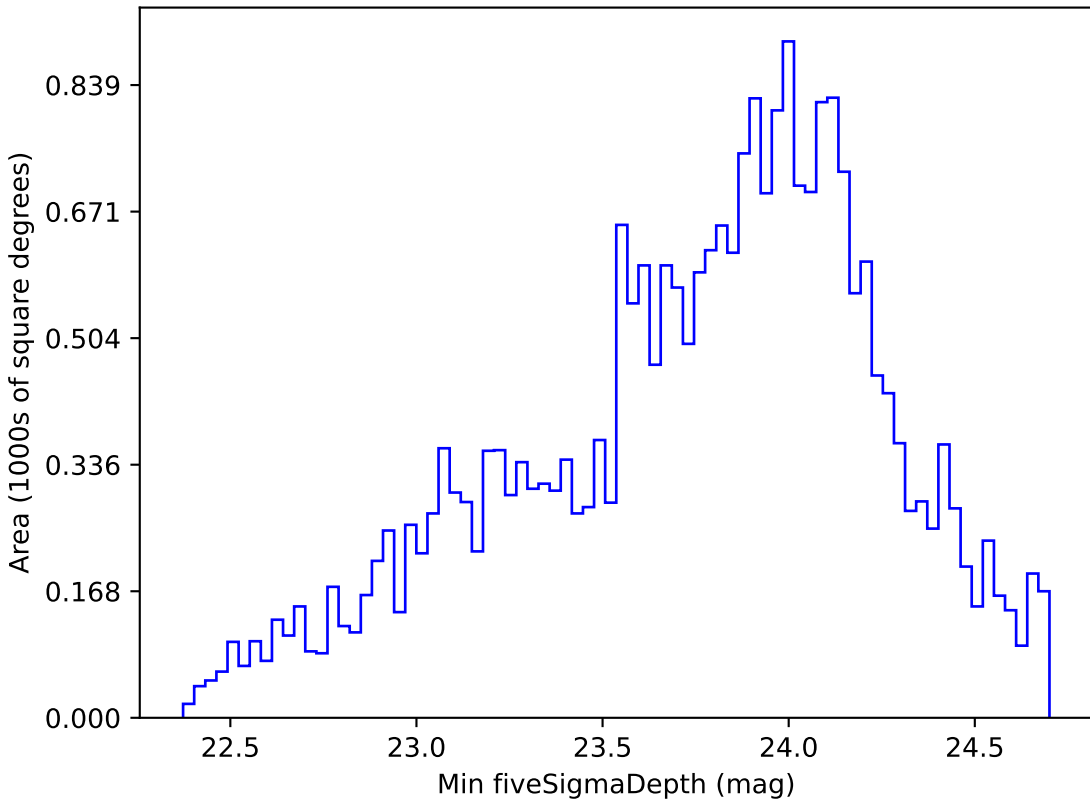
baseline_v3.5_10yrs Yr 1 g band: Min fiveSigmaDepth
