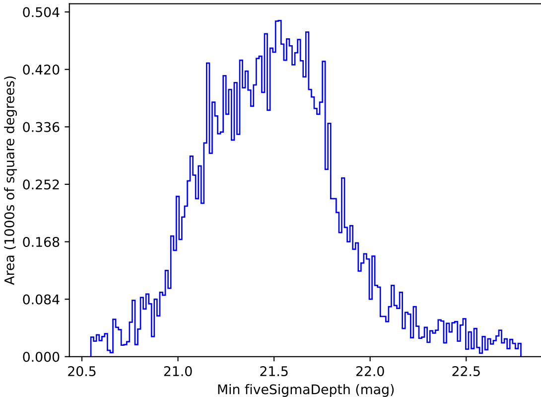
baseline_v3.5_10yrs Yr 1 all bands: Min fiveSigmaDepth
