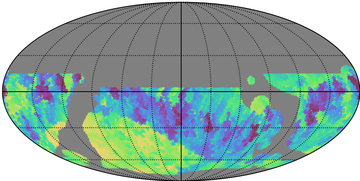
baseline_v3.5_10yrs WFD z band: Min fiveSigmaDepth
