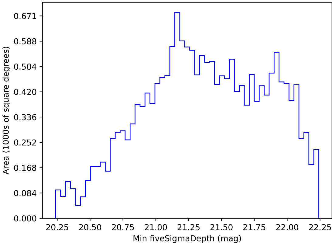
baseline_v3.5_10yrs WFD z band: Min fiveSigmaDepth
