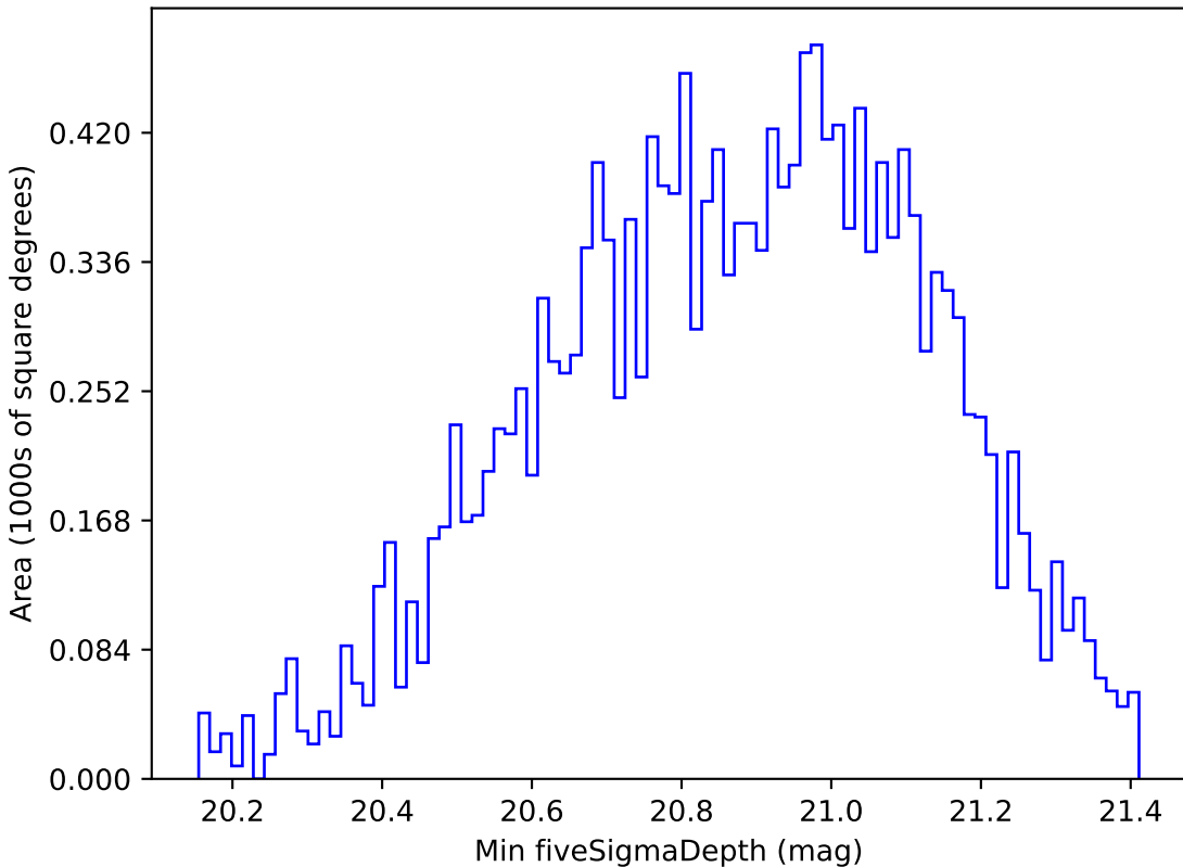
baseline_v3.5_10yrs WFD y band: Min fiveSigmaDepth
