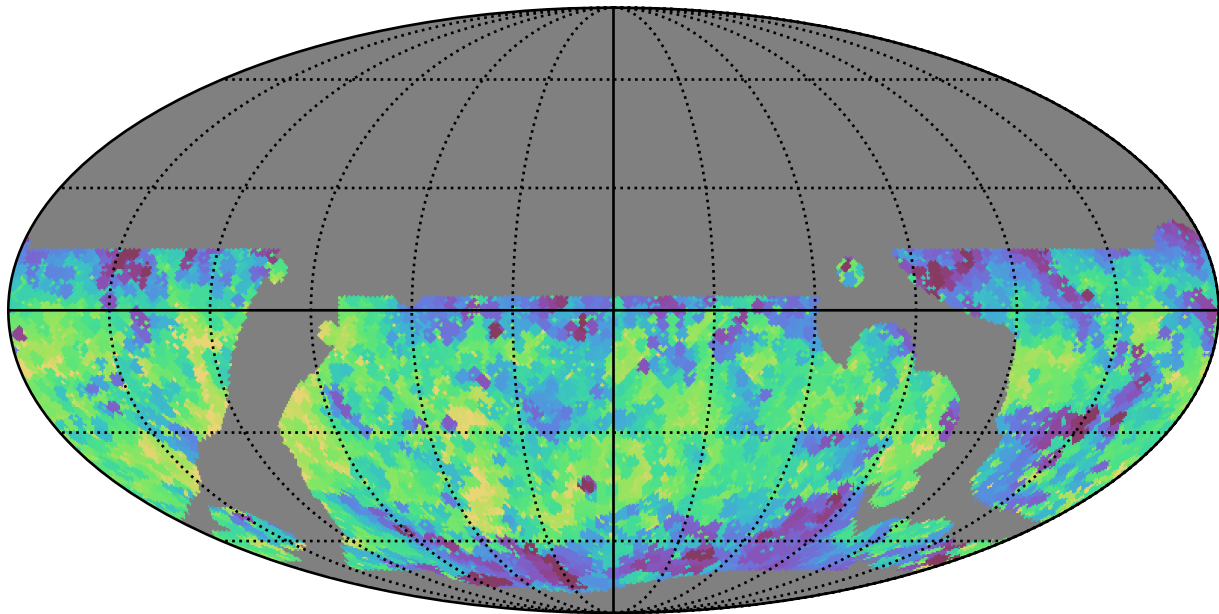
baseline_v3.5_10yrs WFD u band: Min fiveSigmaDepth
