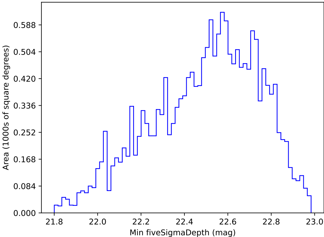
baseline_v3.5_10yrs WFD u band: Min fiveSigmaDepth
