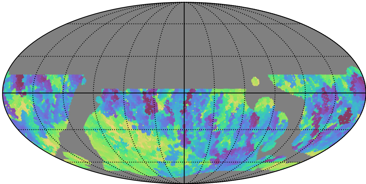
baseline_v3.5_10yrs WFD r band: Min fiveSigmaDepth
