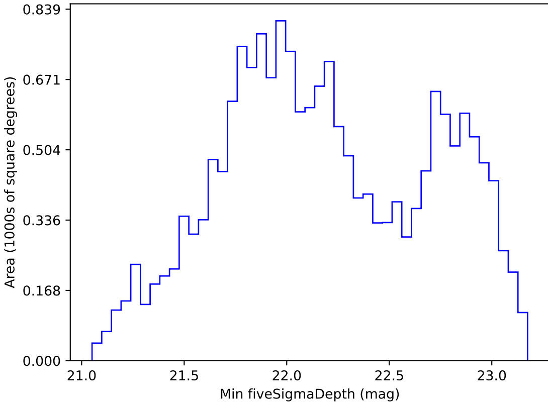
baseline_v3.5_10yrs WFD r band: Min fiveSigmaDepth
