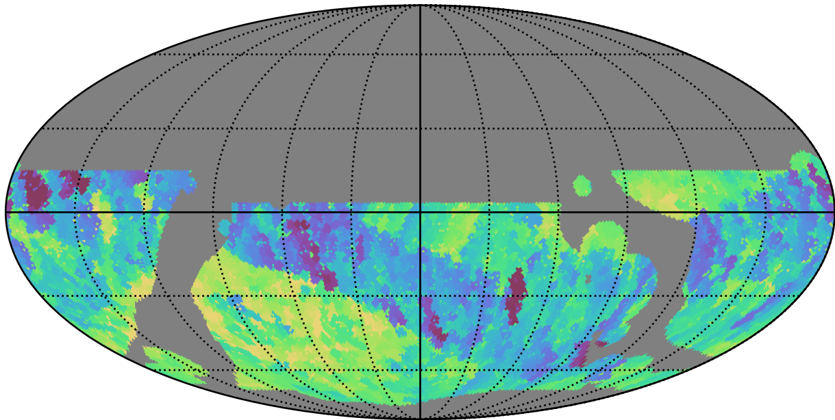
baseline_v3.5_10yrs WFD i band: Min fiveSigmaDepth
