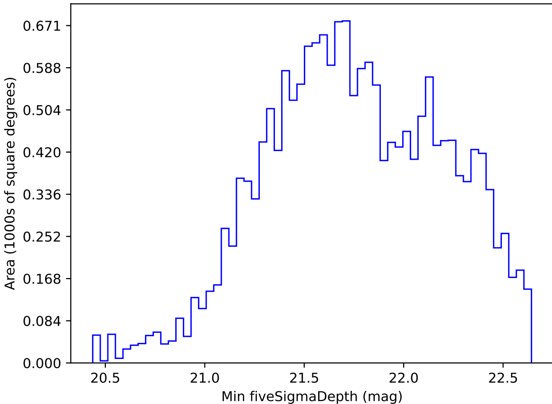
baseline_v3.5_10yrs WFD i band: Min fiveSigmaDepth
