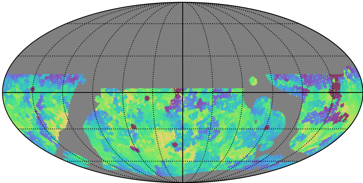
baseline_v3.5_10yrs WFD g band: Min fiveSigmaDepth
