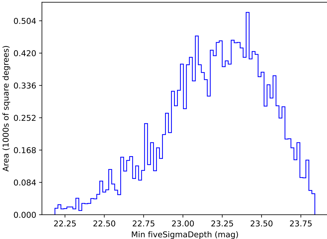
baseline_v3.5_10yrs WFD g band: Min fiveSigmaDepth
