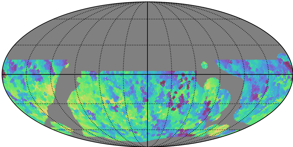
baseline_v3.5_10yrs WFD all bands: Min fiveSigmaDepth
