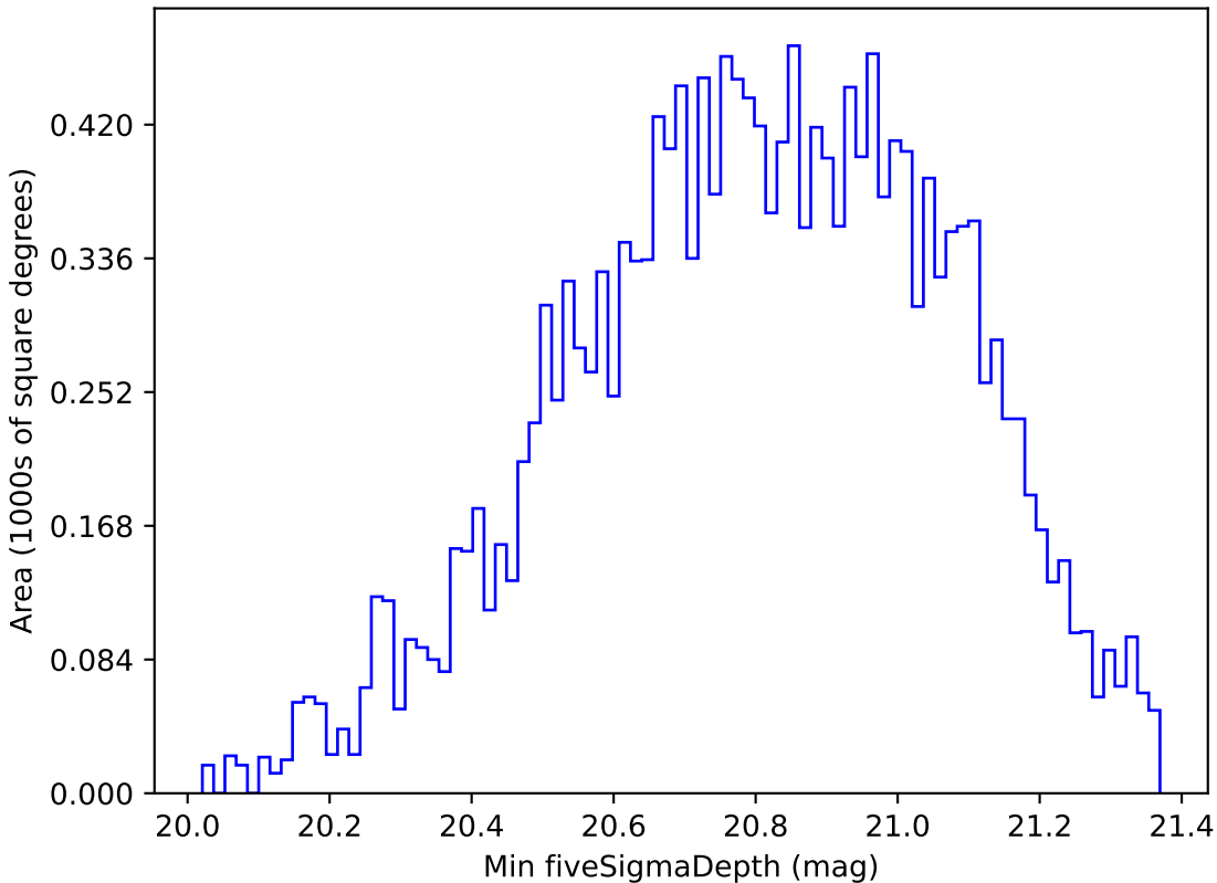
baseline_v3.5_10yrs WFD all bands: Min fiveSigmaDepth
