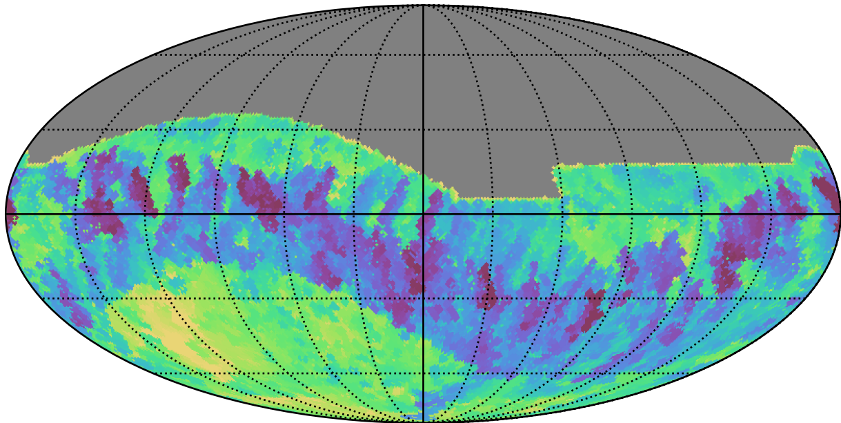
baseline_v3.5_10yrs All sky z band: Min fiveSigmaDepth
