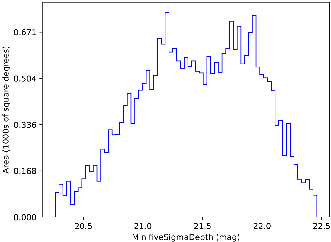
baseline_v3.5_10yrs All sky z band: Min fiveSigmaDepth
