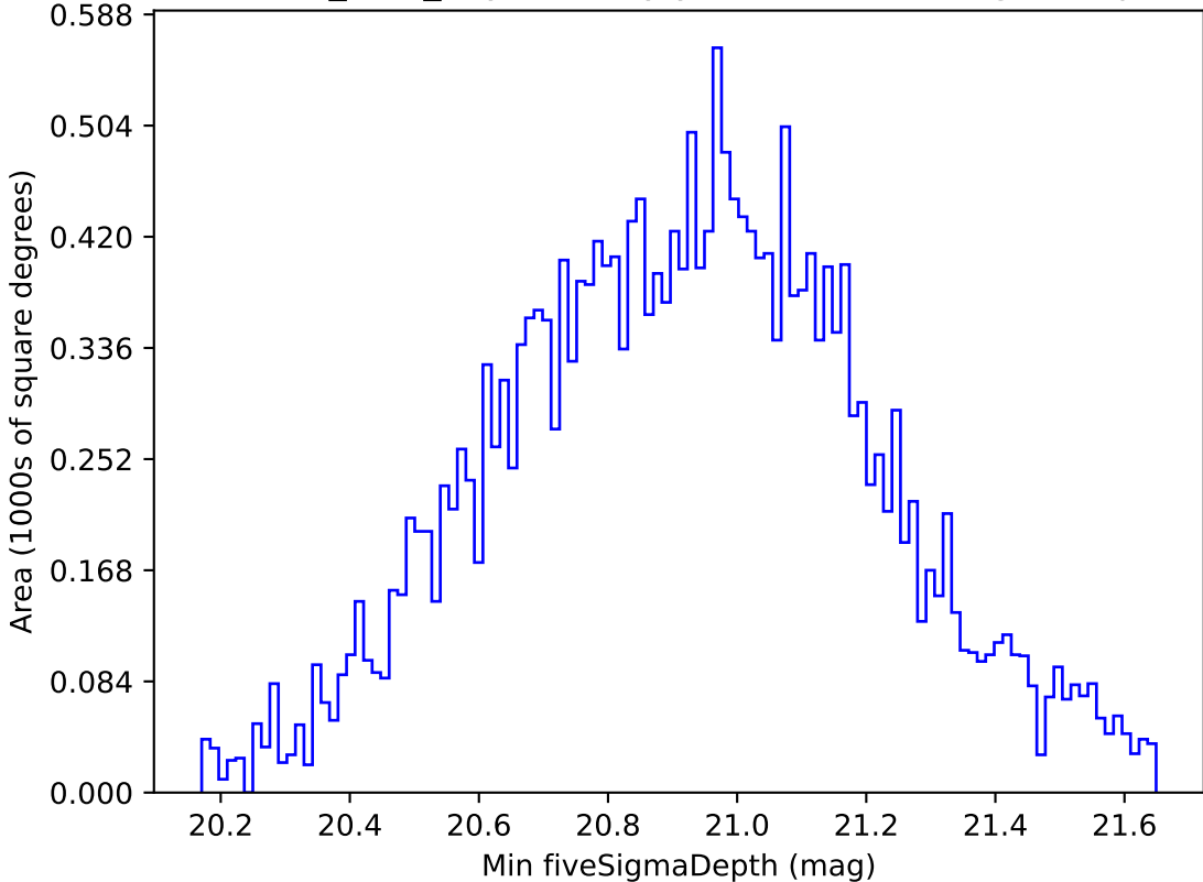
baseline_v3.5_10yrs All sky y band: Min fiveSigmaDepth
