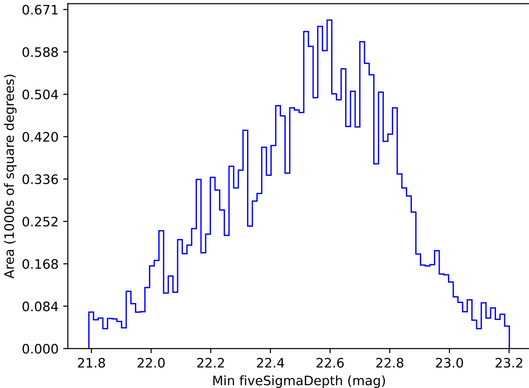
baseline_v3.5_10yrs All sky u band: Min fiveSigmaDepth
