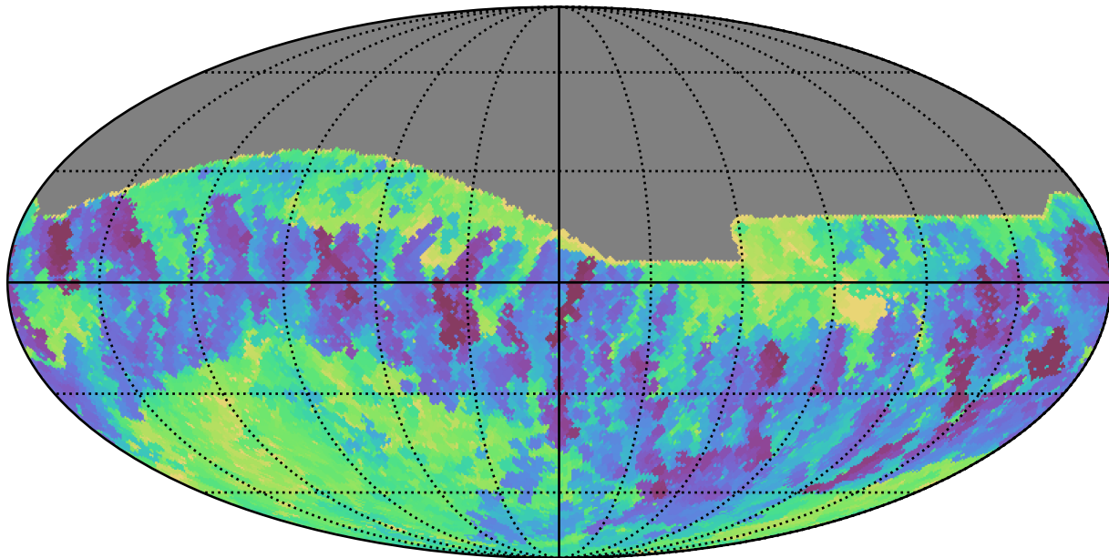
baseline_v3.5_10yrs All sky r band: Min fiveSigmaDepth
