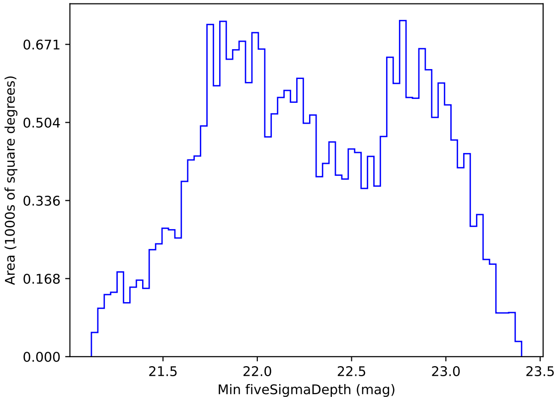
baseline_v3.5_10yrs All sky r band: Min fiveSigmaDepth
