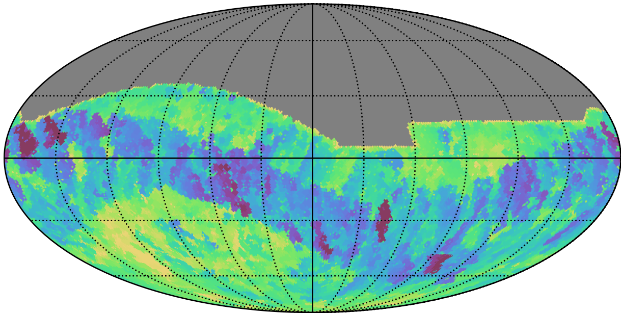
baseline_v3.5_10yrs All sky i band: Min fiveSigmaDepth
