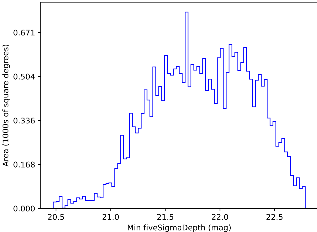
baseline_v3.5_10yrs All sky i band: Min fiveSigmaDepth
