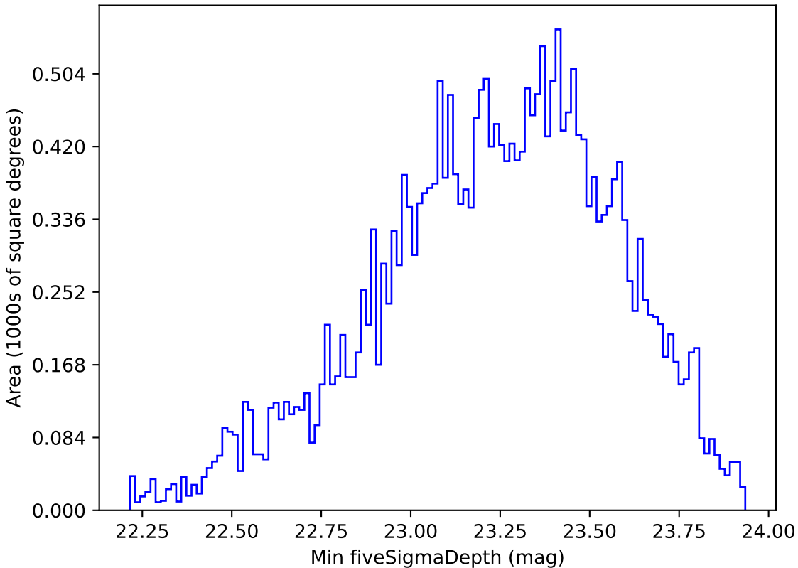
baseline_v3.5_10yrs All sky g band: Min fiveSigmaDepth
